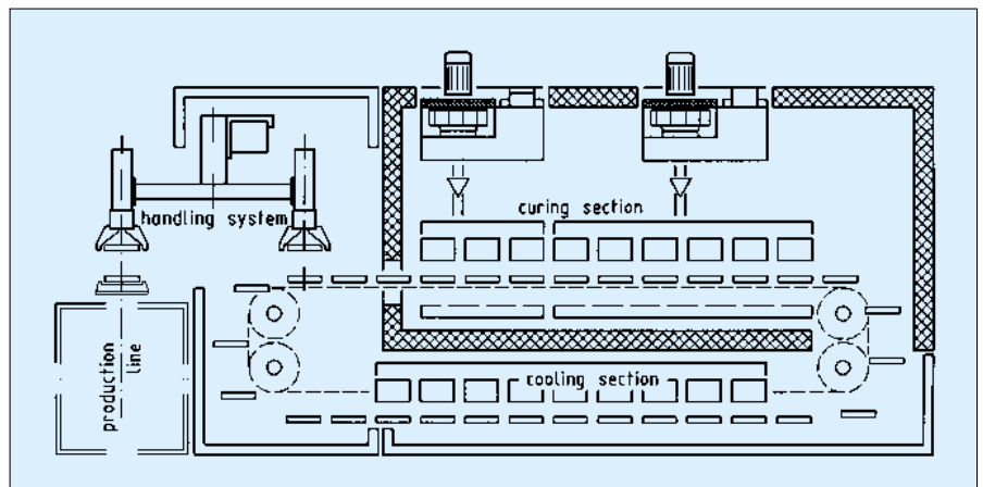
Figure 2: Working principle of a gelling and hardening plant
