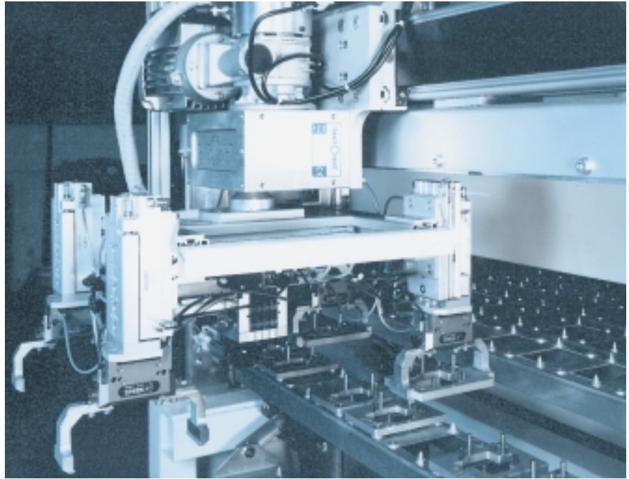
Figure 3: Rotary-type handler with twin gripper
