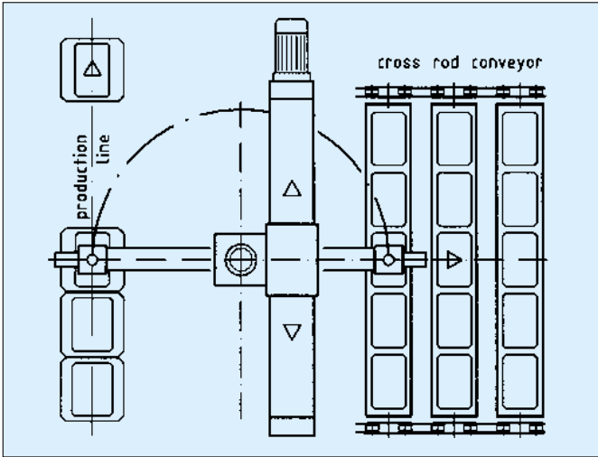
Figure 4: Rotory-type handling principle
